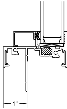
STANDARD 1" SET BACK
