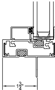
APPLIED 1-3/4" SET BACK
