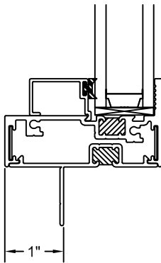
APPLIED 1" SET BACK
