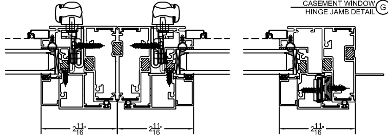
CASEMENT WINDOW HINGE JAMB DETAIL G
