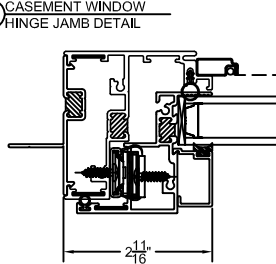
F CASEMENT WINDOW HINGE JAMB DETAIL
