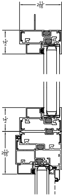
A HEAVY PICTURE WINDOW HEADER DETAIL
