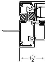
C HEAVY PICTURE WINDOW LEFT JAMB DETAIL
