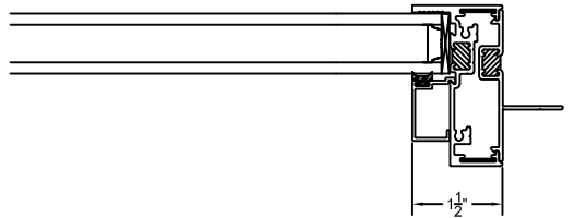
HEAVY PICTURE WINDOW RIGHT JAMB DETAIL D
