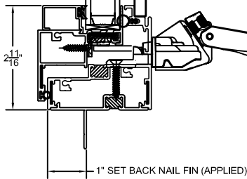
B AWNING WINDOW SILL DETAIL
