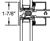
(B) HEAVY PICTURE WINDOW HOLLOW MUNTIN DETAIL
