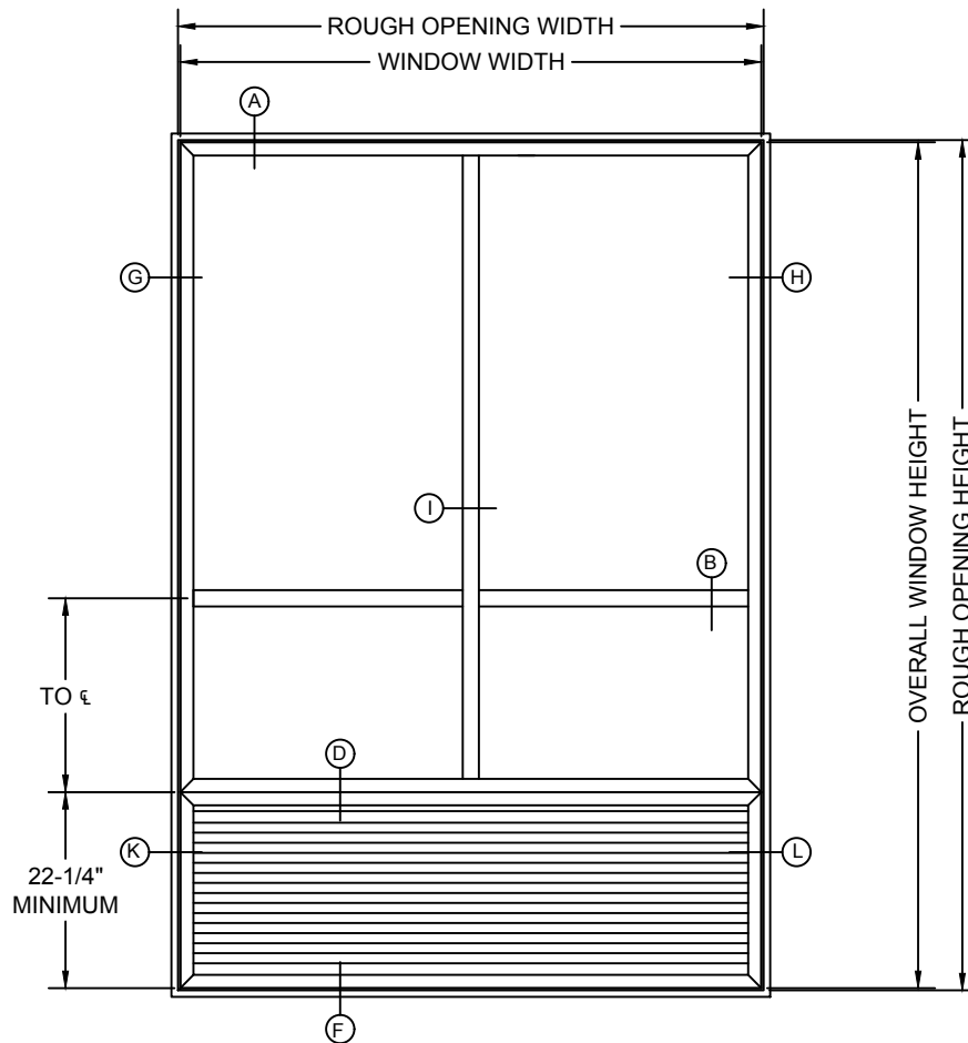
Ⓜ HEAVY PICTURE WINDOW HOLLOW MUNTIN DETAIL
