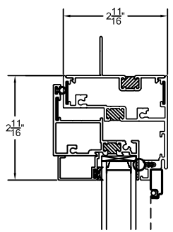
A CASEMENT WINDOW HEADER DETAIL
