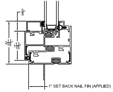
D FIXED CASEMENT WINDOW SILL DETAIL
