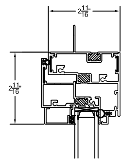
B FIXED CASEMENT WINDOW HEADER DETAIL
