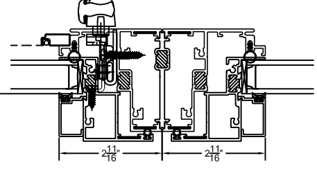
D CASEMENT WINDOW LOCKING/FIXED JAMB DETAIL
