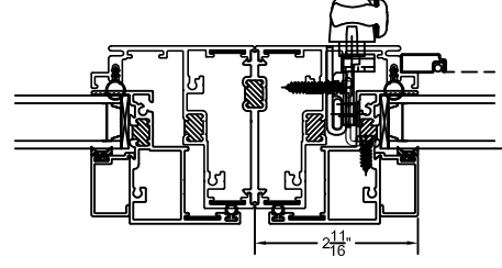
CASEMENT WINDOW FIXED/LOCKING JAMB DETAIL E
