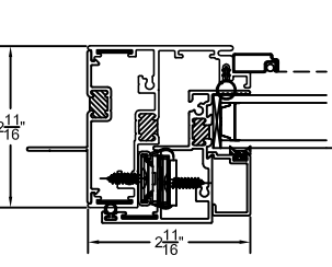
C CASEMENT WINDOW HINGE JAMB DETAIL
