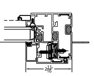
CASEMENT WINDOW F HINGE JAMB DETAIL
