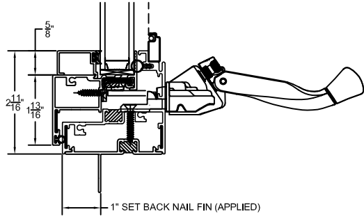
C CASEMENT WINDOW SILL DETAIL
