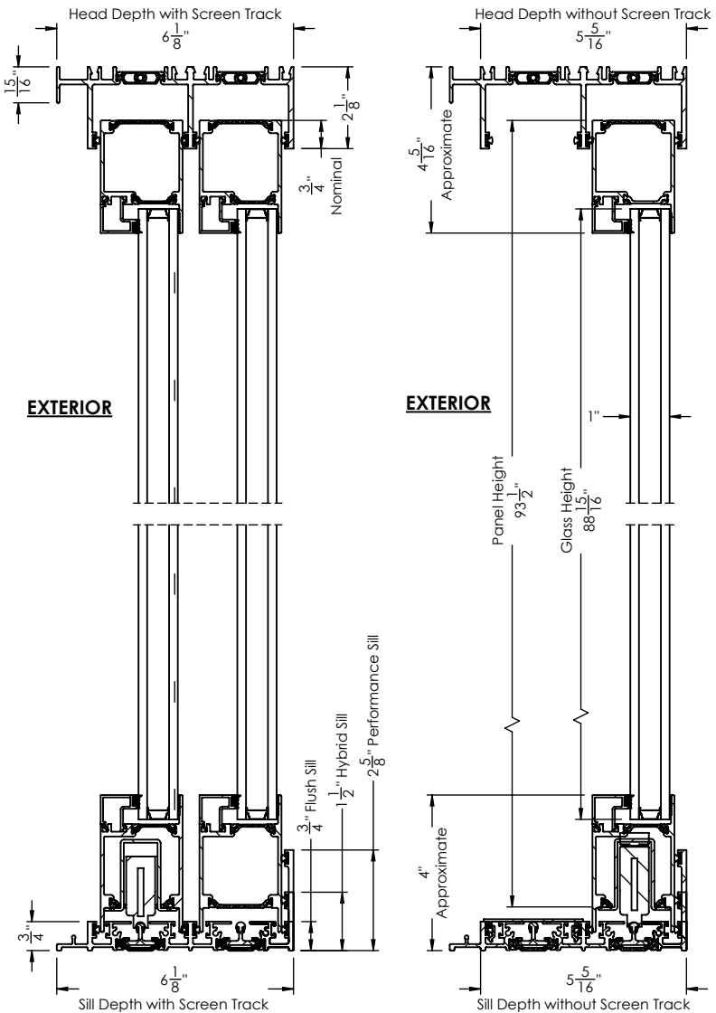
SECTION B-B SCALE 1 : 4.5
